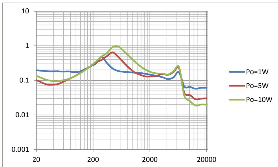
THD+N vs Frequency, V_{CC}=18V , R_L= 8\ \Omega BTL
