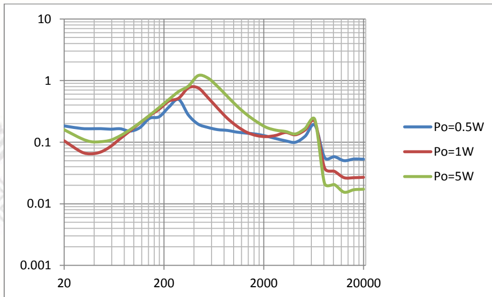
THD+N vs Frequency, V_{CC}=12V , RI= 8 BTL
